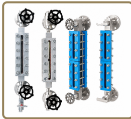
Reflex Level Indicator
